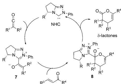
Scheme 5. Proposed mechanism.
