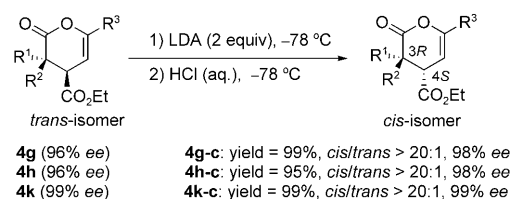
Scheme 1. Synthesis of cis -δ-lactones from trans -δ-lactones.
