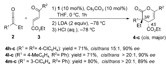
Scheme 2. Synthesis of cis -δ-lactones from ketene–enone cycloaddition.
