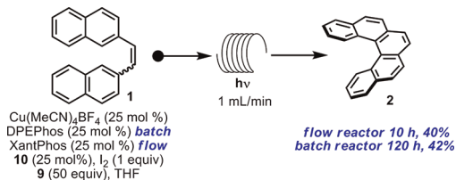
Scheme 1. Scale-up Synthesis of [5]Helicene Using Either a Round Bottom Flask or Continuous Flow Strategy
