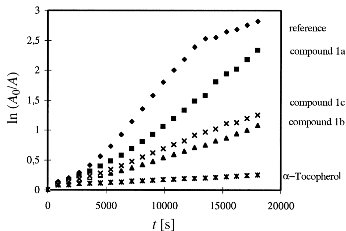
Fig. 3. Determination of K = K_0/K by using the slopes at the beginning of reactions for 1a , 1b , and 1c , and \alpha -tocopherol ( K ) and without antioxidant ( K_0 )
