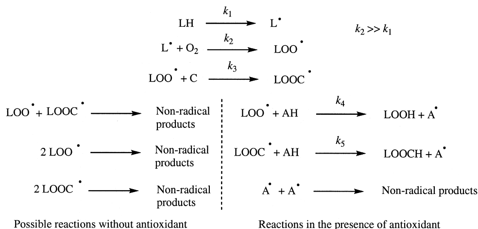
Scheme 1. Possible Reactions with and without Antioxidant ( k_1, k_2, k_3, k_4 , and k_5 are reaction rates, LH = linoleic acid, C = \beta -carotene)
