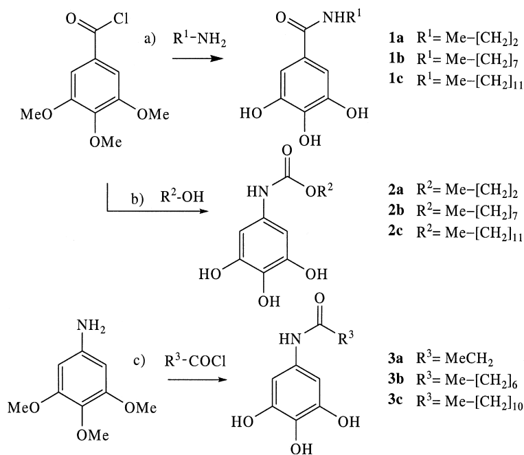
Scheme 2. Synthesis of Hydrophobic Gallic Acid Derivatives
