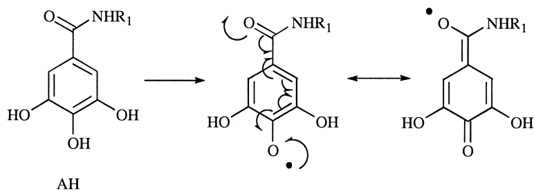
Scheme 3. Stabilization of the Phenoxy Radical by Electron Delocalization
