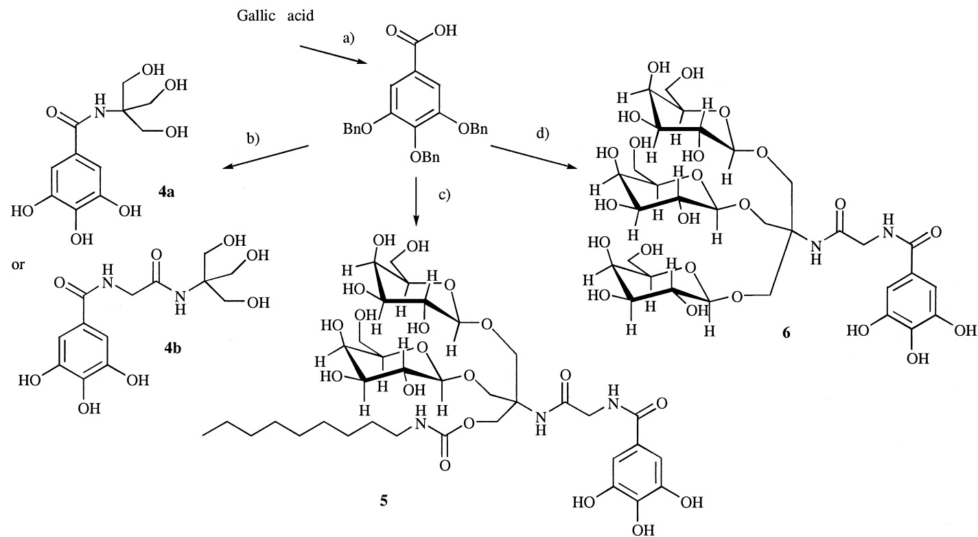
Scheme 4. Synthesis of Hydrophilic Gallic Acid Derivatives
