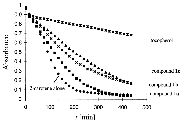
Fig. 2. Kinetics of the \beta -carotene oxidation in the presence of N -alkyl amides 1a , 1b , and 1c , or \alpha -tocopherol
