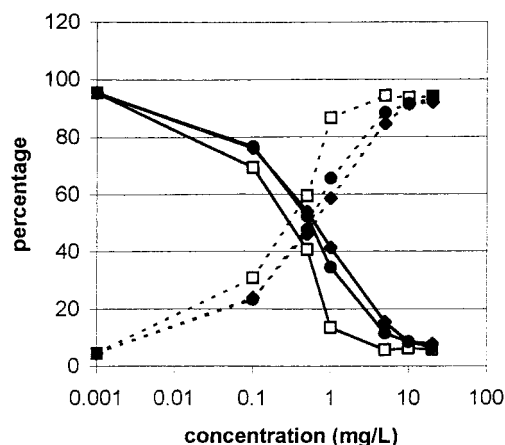
Figure 3. Sterol composition of U. maydis sporidia (ATCC 14826) after 18 h of treatment with increasing concentrations of racemic 4a , (+)- 4a , and (-)- 4a added to actively growing cultures: (—) 14 \alpha -demethylsterols; (---) 14 \alpha -methylsterols; (●) racemic 4a ; (□) (+)- 4a ; (◆) (-)- 4a .
