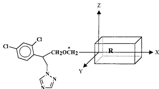
Figure 2. Definition of some of the parameters of Table 3. Geometrical descriptors: |X|_{\max} = X1 ; |Y|_{\max} = Y1 ; |Y|_{\min} = Y2 ; |Z|_{\max} = Z1 ; |Z|_{\min} = Z2 . Charge: * indicates the carbon used for the charge.
