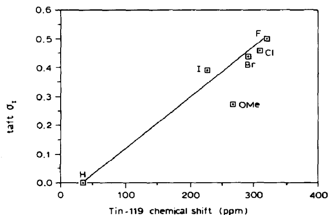
Fig. 1. Plot of ^{119}\text{Sn} NMR chemical shift ( \delta in ppm) vs Taft \sigma_1 constant for the series [\text{FeCp}(\text{CO})_2\{\text{Sn}(\text{X})\text{R}_2\}] ( \text{X} , \sigma_1 = \text{H} , 0.00; F, 0.50; Cl, 0.46; Br, 0.44; I, 0.39; OMe, 0.27).
