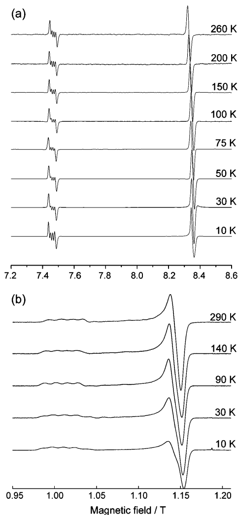
Figure 5. (a) 244 GHz single-crystal EPR spectra of [Cu(hfac) 2 (PPz Et )] at T = 10–260 K ( \nu_{mw} \approx 243.68 GHz, arbitrary crystal orientation). (b) Q-band powder EPR spectra of [Cu(hfac) 2 (PPz Et )] at T = 10–290 K ( \nu_{mw} \approx 33.21 GHz). The temperature values are given on the right.
