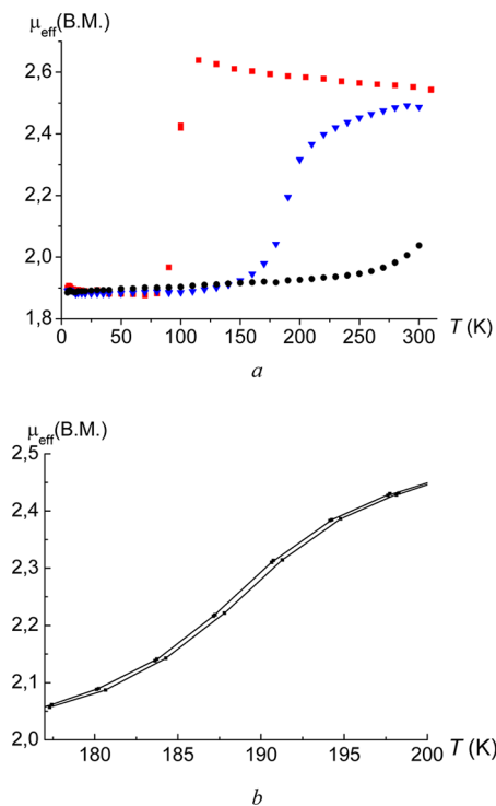
Figure 3. Experimental dependences \mu_{\text{eff}}(T) for [\text{Cu}(\text{hfac})_2(\text{NPz}^{\text{Me}})] (red ■), [\text{Cu}(\text{hfac})_2(\text{NPz}^{\text{Et}})] \cdot 0.5\text{C}_7\text{H}_{16} (blue ▼), and [\text{Cu}(\text{hfac})_2(\text{NPz}^{\text{Pr}})] (●) at 1.0 T (a) and hysteresis for [\text{Cu}(\text{hfac})_2(\text{NPz}^{\text{Et}})] \cdot 0.5\text{C}_7\text{H}_{16} (b).
