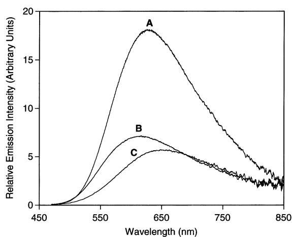
Fig. 4. Corrected emission spectra of \text{Mo(CO)}_4(\text{Cmic})_2 (A); \text{Mo(CO)}_4(\text{Mic})_2 (B); and \text{Mo(CO)}_4(\text{Dmic})_2 (C) in \text{CH}_2\text{Cl}_2 solution.
