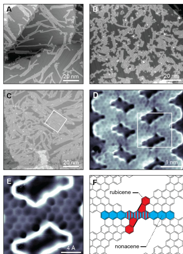
Figure 1. Synthesis of C-NPG. (A) STM topographic image of 0.25 monolayer coverage of C-NPG on Au(111) after deposition of 2 onto Au(111) held at T_1 = 180 °C and subsequent annealing to T_2 = 400 °C ( V = 1.2\text{ V} , I = 50\text{ pA} ). (B) STM topographic image of 0.75 monolayer coverage of C-NPG on Au(111) after deposition of 1 onto Au(111) held at 24 °C and subsequent annealing to T_2 = 400 °C ( V = -1.2\text{ V} , I = 50\text{ pA} ). (C) STM topographic image of 0.75 monolayer coverage of C-NPG on Au(111) after deposition of 2 onto Au(111) held at T_1 = 180 °C and subsequent annealing to T_2 = 400 °C ( V = 1.2\text{ V} , I = 50\text{ pA} ). (D) Bond-resolved STM image of a region containing three fused ribbons ( V = -50\text{ mV} , I = 200\text{ pA} , V_{\text{osc}} = 15\text{ mV} , f = 620\text{ Hz} ). (E) High-resolution bond-resolved STM image of the region indicated in (D) ( V = 20\text{ mV} , I = 250\text{ pA} , V_{\text{osc}} = 10\text{ mV} , f = 620
