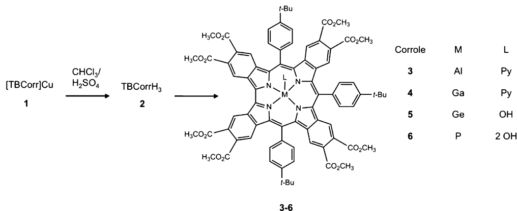
Scheme 1. Synthetic Pathway for the Preparation of meso -Triaryltetrabenzocorrole Metal Complexes
