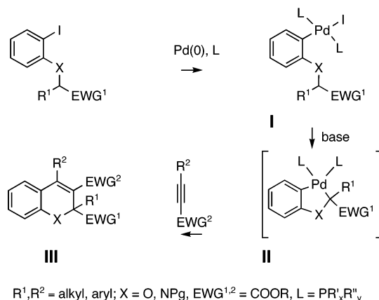
R 1 , R 2 = alkyl, aryl; X = O, NPg, EWG 1,2 = COOR, L = PR x R y Figure 1. Synthetic strategy.
