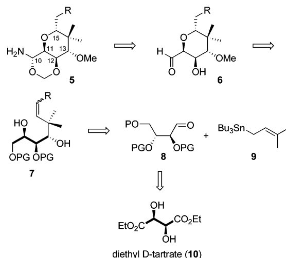
SCHEME 2. Retrosynthetic Analysis of the Right Part of Mycalamides
