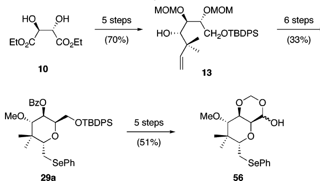
SCHEME 18. Overall Sequence for Synthesis of Trioxadecalin 56 from Diethyl D-Tartrate
