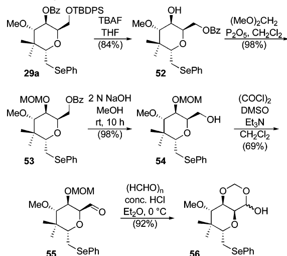
SCHEME 17. Formation of Trioxadecalin 56, the B,C-Ring System of Mycalamides
