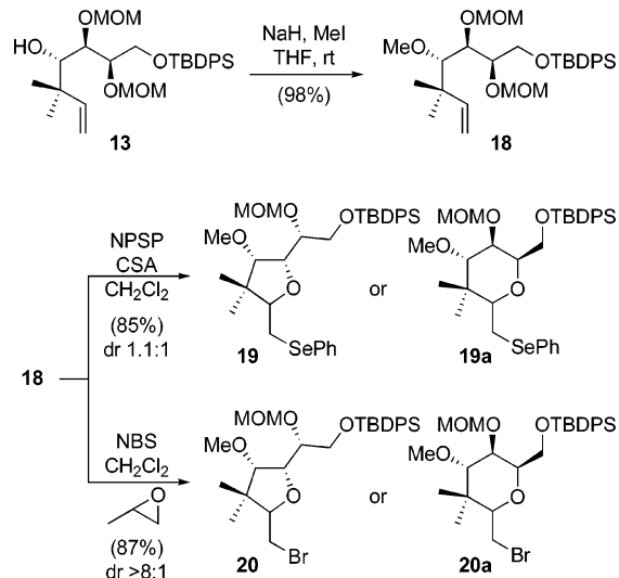
SCHEME 6. Electrophilic Cyclization of Bis-MOM Alkene 18
