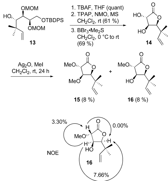
SCHEME 4. Determination of Stereochemistry of Addition Product 13
