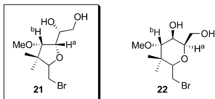
FIGURE 3. Determination of the structure of cyclization product by ^1\text{H} NMR decoupling pattern of the derivative of 21 or 22 .
