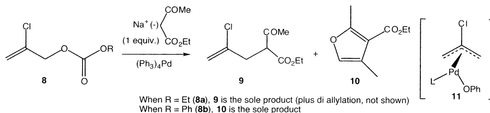
FIGURE 2. Attack of sodium ethyl 3-oxobutanate on a 2-Cl \pi -allyl Pd complex.
