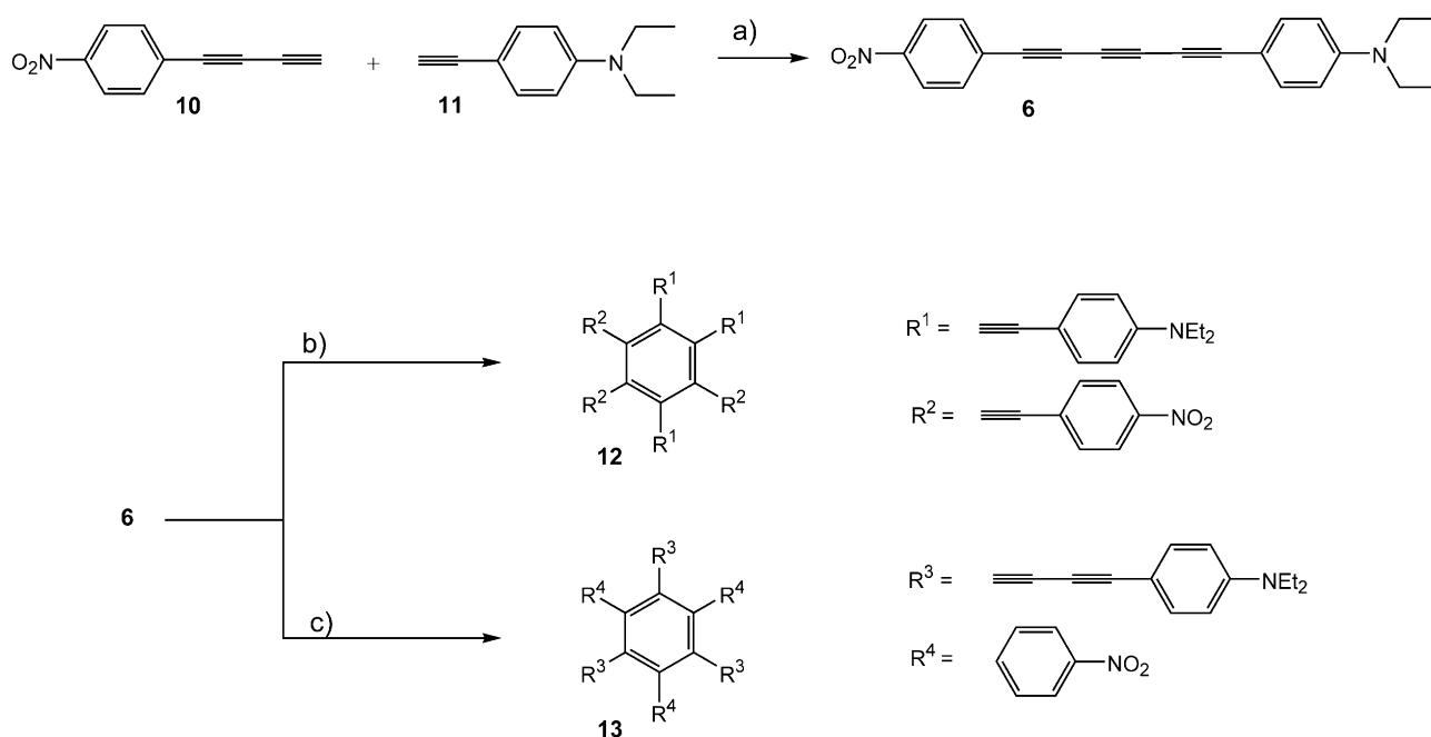
Scheme 4. a) \text{CuCl} , TMEDA, \text{O}_2 ; b) [\text{Ni}(\text{PPh}_3)_2(\text{CO})_2] ; c) [\text{Rh}(\text{PPh}_3)_3\text{Cl}] .
