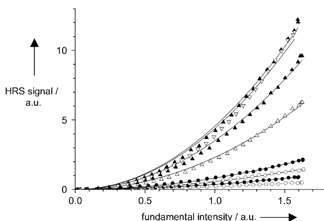
Figure 6. HRS signals S^{2\omega} as a function of the fundamental intensity I^\omega of 3 (circles, c=1.3, 2.7, 5.4, 11.0 \text{ mol m}^{-3} ) and 4b (triangles, c=0.10, 0.19, 0.39, 0.80 \text{ mol m}^{-3} ) in 1,4-dioxane for increasing concentration c .
