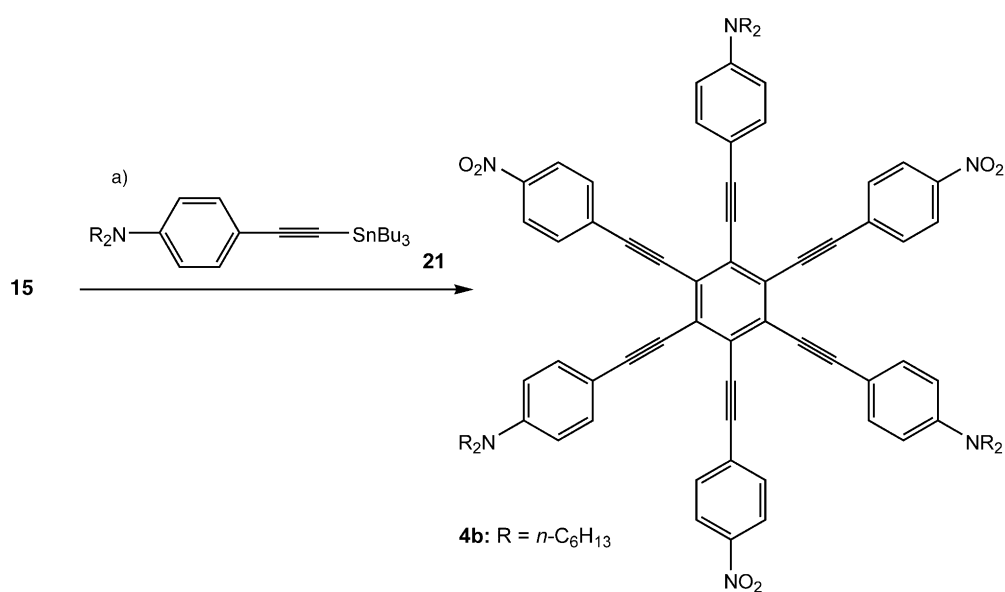
Scheme 7. a) [\text{Pd}(\text{PPh}_3)_4] , CuO, 21 , DMF, 98^\circ\text{C} .
