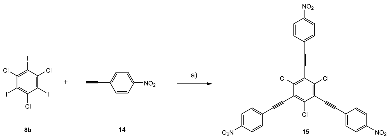
Scheme 5. a) [\text{Pd}(\text{PPh}_3)_4] , CuI, \text{HN}(\text{iC}_3\text{H}_5)_2 , THF.
