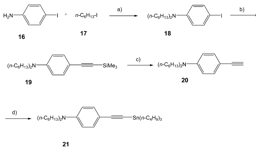
Scheme 6. a) \text{Na}_2\text{CO}_3 , DMF, 120^\circ\text{C} , 20 h; b) \text{HC}\equiv\text{C-SiMe}_3 , [\text{Pd}(\text{PPh}_3)_4] , CuI, \text{HNEt}_2 ; c) KOH, \text{H}_2\text{O}/\text{EtOH} , d) n\text{BuLi}/\text{THF} , (n\text{C}_4\text{H}_9)_3\text{SnCl} .
