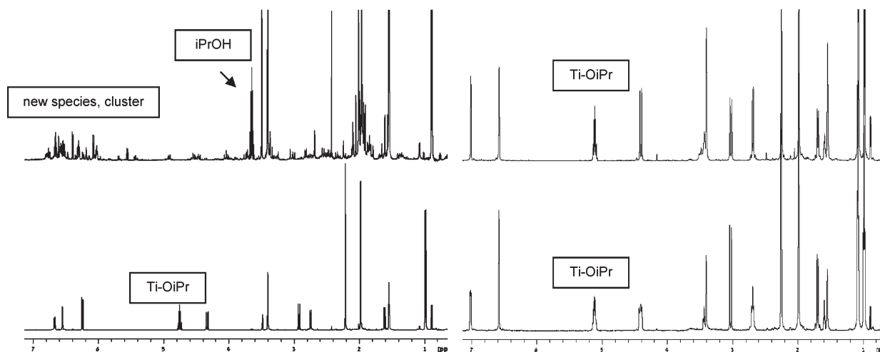
Figure 4. ^1\text{H} NMR spectra of \text{L}^5\text{Ti}(\text{OiPr})_2 (left) and \text{L}^7\text{Ti}(\text{OiPr})_2 (right) at RT in d_8 -THF immediately (bottom) and 20 h (top) following addition of \text{D}_2\text{O} .
