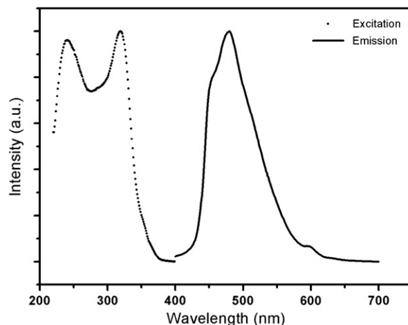
Fig. 3. Excitation (left) and emission (right) spectrum of the compound (I).
