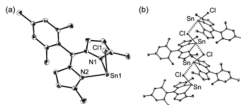
Figure 1. (a) ORTEP drawing of 2 (50% probability). (b) Packing structure of 2 . For selected distances and angles, see the Supporting Information.
