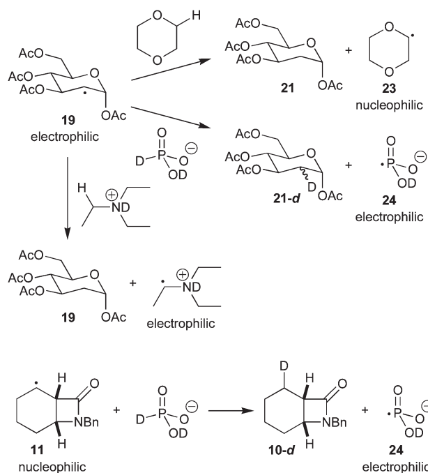
Scheme 7 Polar effects in H/D-atom abstraction.
