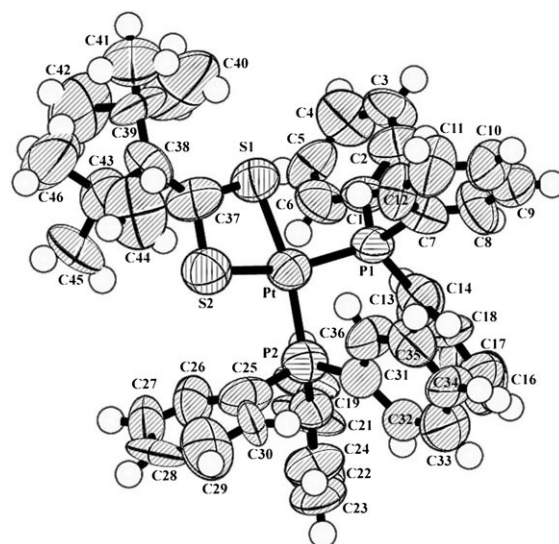
Figure 2. ORTEP drawing of complex 22 . Bond lengths: C37–S1: 1.790(3), C37–S2: 1.780(3), Pt–S1: 2.290(7), and Pt–S2: 2.283(8) Å. Bond angles: S2–C37–S1: 103.4(14), S2–Pt–S1: 75.6(3), C37–S1–Pt: 90.2(9), and C37–S2–Pt: 90.7(10)°.
