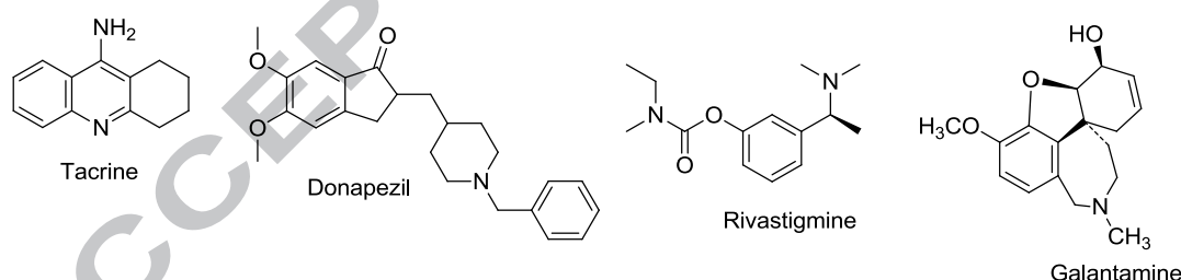
Fig. 1. Structures of approved AChE inhibitors.
