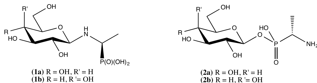
Figure 1. N -Linked and O -linked glycoside and galactoside targets
