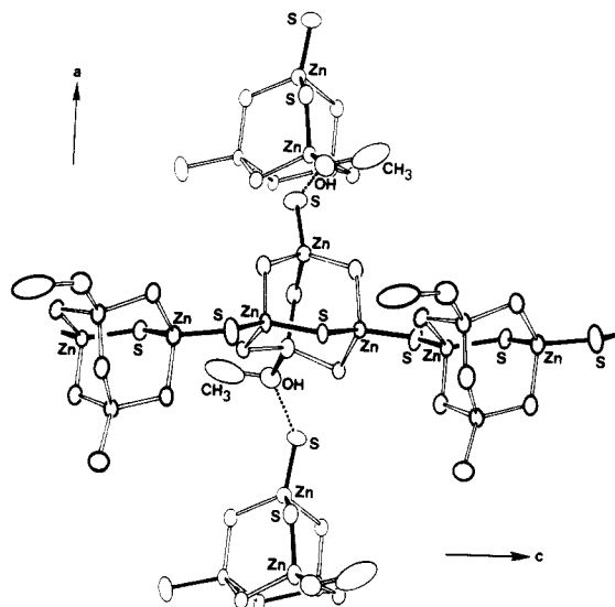
Figure 1. Crystal structure of \text{Zn}_4(\text{SPh})_8\text{MeOH} (1).
