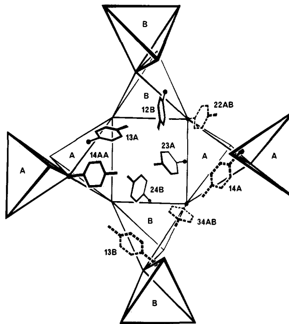
Figure 9. Representation of the adamantanoid tetrahedra that surround the cavity in 3 and of the 4-methylbenzenethiolate ligands that are located in or near the cavity. For clarity, the four adamantanoid tetrahedra of the top four-membered ring have been omitted, as have ligands related by inversion through the center of the cavity. The five independent ligands that protrude into the cavity are drawn with solid lines; those four that are approximately tangential to the surface of the cavity are drawn with broken lines.
