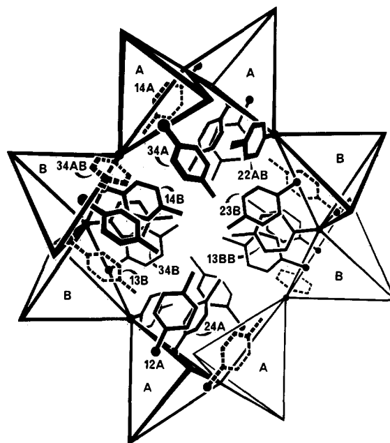
Figure 10. Representation of the ligands on a centrosymmetric eight-membered ring of adamantanoid tetrahedra surrounding the channel in the crystal structure of 3 . The 4-methylbenzenethiolate ligands that protrude into the channel are drawn with solid lines, and those tangential to the channel are drawn with broken lines.
