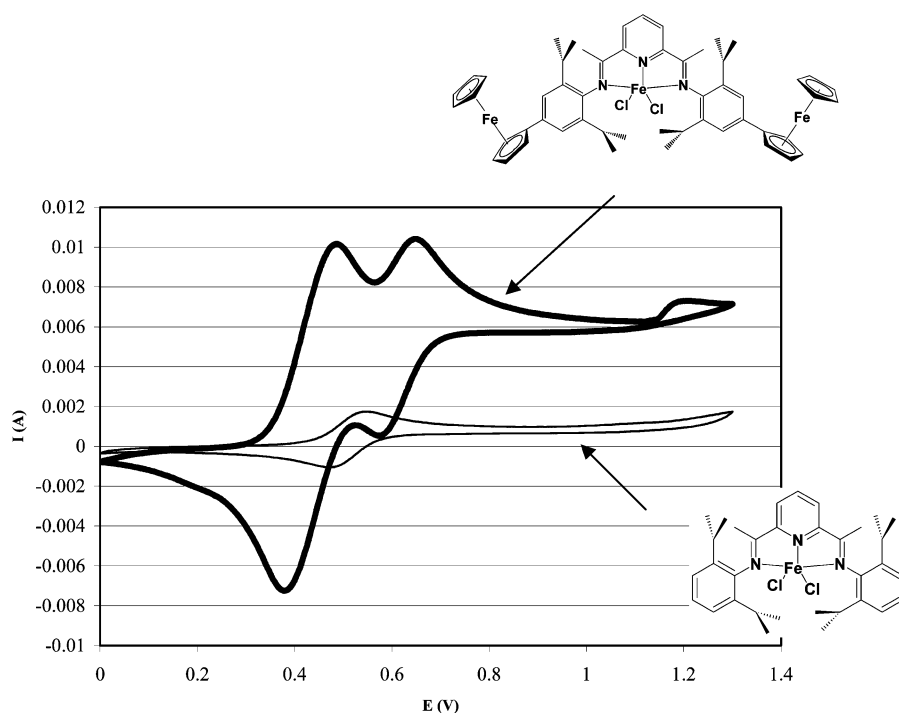
Figure 3. Comparison of the cyclic voltammograms of the iron complexes FECAT and 7. Conditions: 0.01 M dichloromethane solution of compound; supporting electrolyte 0.1 M n\text{Bu}_4\text{NPF}_6 . Standard calomel electrode as reference electrode with palladium working and auxiliary electrodes. Scan rate 100 \text{ mV s}^{-1} .
