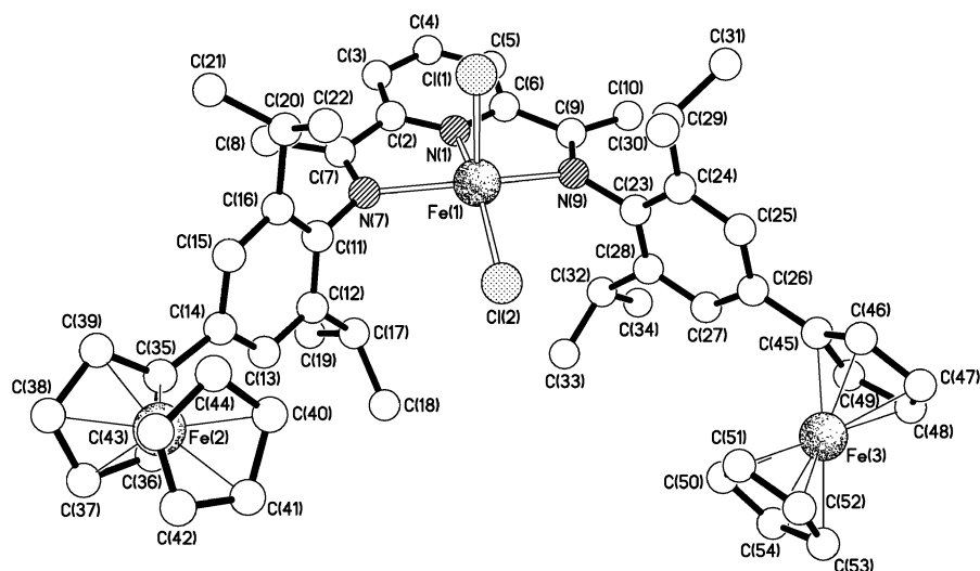
Figure 2. Molecular structure of 7.
