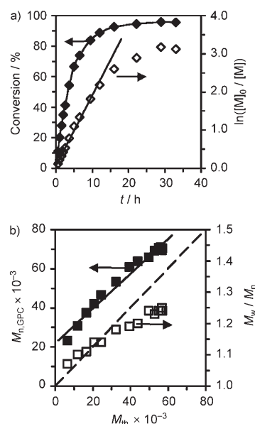
Figure 3. Polymerization of (3,4-3,5)12G2-4EBn with Rh(C\equiv CPh)(nbd)-(PPh_3)_2/DMAP in THF at 23 °C; [EBn]_0/[Rh]_0/[DMAP]_0 = 50:1:10 , [M]_0 = 0.052 M. a) Plot of conversion ( \blacklozenge ) and first-order logarithm ( \ln([M]_0/[M]) , \diamond ) versus time for the same reaction. b) Plot of experimental M_{n,GPC} (GPC vs PS standards) ( \blacksquare ) and M_w/M_n ( \square ) versus M_{th} .
