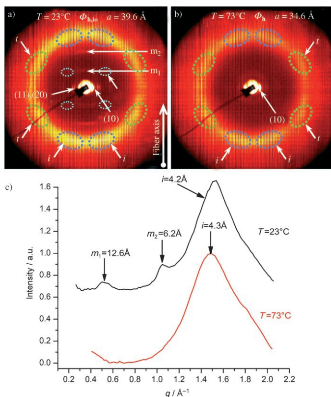
Figure 7. Wide angle X-ray diffraction patterns from poly[(3,4,5)12G1-4EBn] collected at a) 23^\circ\text{C} and b) 73^\circ\text{C} , and c) the corresponding stack meridional plots. Legend: i -short range helical feature; t - 54 \pm 9^\circ dendron tilt angle; m_1 and m_2 -meridional helical features; h_1 -long range helical feature; (10), (11) and (20)-( hk0 ) reflections of the columnar hexagonal phase.
