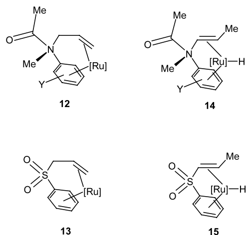
Fig. 4. The co-ordination of ruthenium to benzene ring might be an important factor to Z – E regioselectivity. The co-ordination of N -allylamides and N -(1-propenyl)amides is supported by quantum calculation [41].
