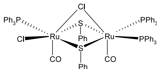
Fig. 1. Structure of chlorocarbonyl(triphenylphosphine)ruthenium (II)- \mu -chloro-di(thiophenolato)-carbonyl-bis(triphenylphosphine)-ruthenium(II)—the yellow complex ( 3 ) isolated from the reaction between allyl phenyl sulphide and [\text{RuClH}(\text{CO})(\text{PPh}_3)_3] .
