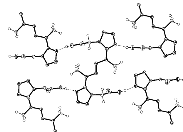
FIGURE 1. Molecular structure and intermolecular hydrogen bonds of 13 . Thermal ellipsoids are drawn at the 50% probability level.
