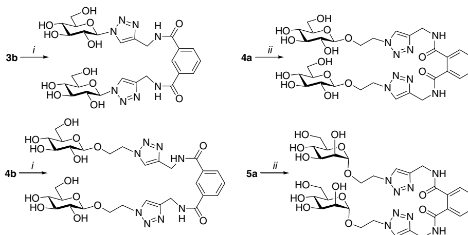
Scheme 3. Reagents and conditions: (i): 7 M \text{NH}_3 in MeOH, 16 h, rt, 99% from 3b , 72% from 4b ; (ii): cat. NaOMe in MeOH, 30 min, rt, 96% from 4a , 98% from 5a .
