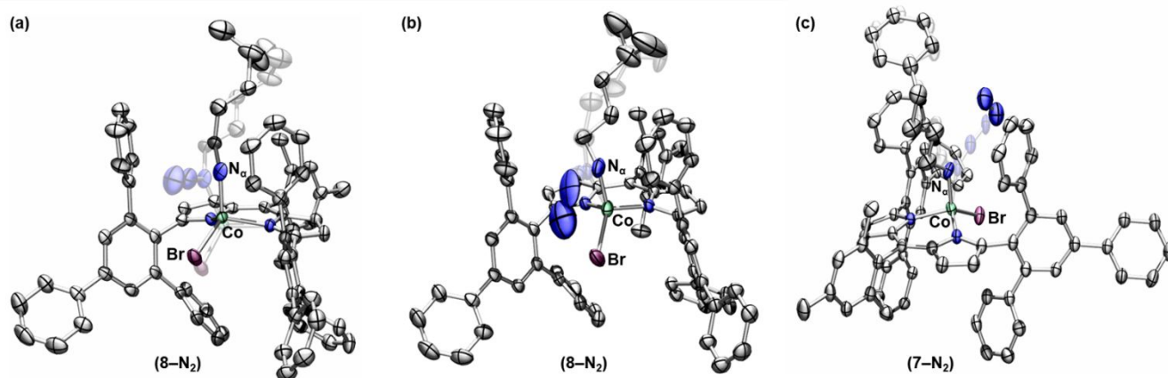
Figure 6. Solid-state structures for (a) 8-N 2 collected at 100 K following heating to 345 K, (b) 8-N 2 , and (c) 7-N 2 collected at 100 K upon X-ray irradiation with thermal ellipsoids at the 50% probability level (hydrogen atoms and solvent molecules are omitted for clarity; Co aquamarine, C gray, N blue, Br maroon).
