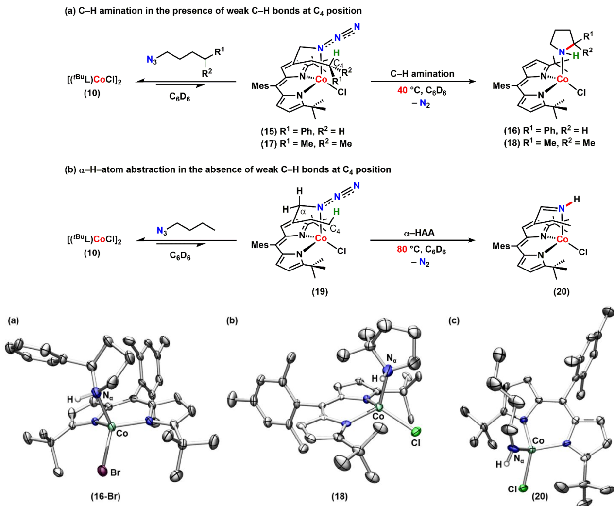
Figure 8. Solid-state structures for (a) 16-Br , (b) 18 , and (c) 20 at 100 K with thermal ellipsoids at the 50 % probability level (hydrogen atoms except for N–H or imine C–H and solvent molecules are omitted for clarity; Co aquamarine, C gray, N blue, Br maroon, Cl green, H white.)
