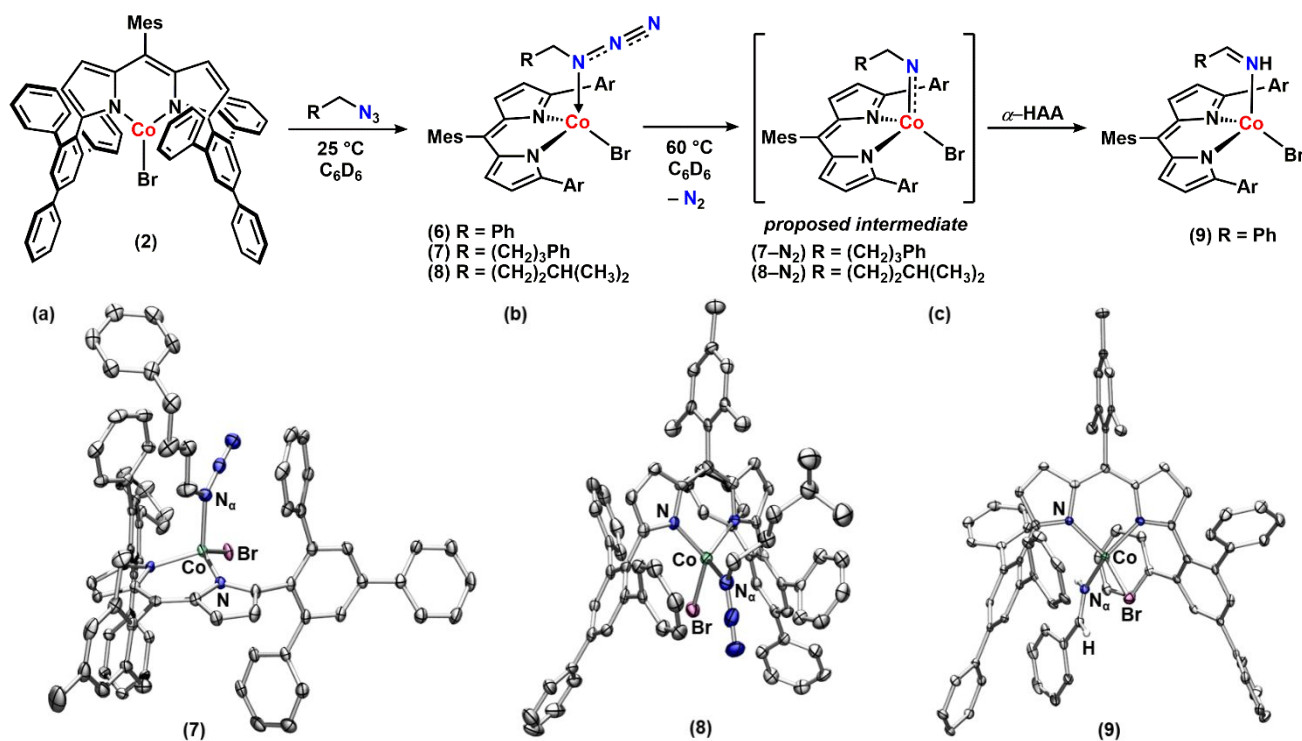
Figure 5. Solid-state structures for (a) 7 , (b) 8 and (c) 9 at 100 K with thermal ellipsoids at the 50% probability level (hydrogen atoms except for imine moiety of 9 and solvent molecules are omitted for clarity; Co aquamarine, C gray, N blue, Br maroon, H white).
