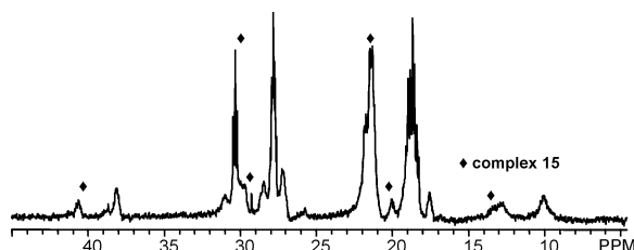
Figure 5. Partial ^{31}\text{P}\{^1\text{H}\} NMR spectrum of the mixture obtained from the reaction of 15 with (p\text{-Tol})_3\text{P} (202 MHz, \text{C}_7\text{D}_8 , 223 K).
