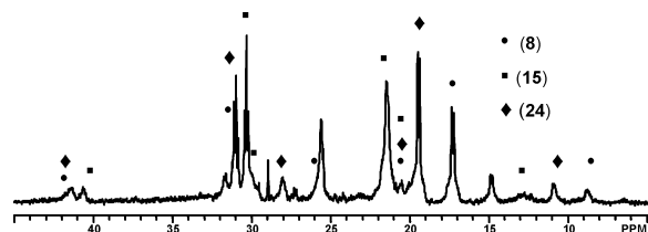
Figure 6. Partial ^{31}\text{P}\{^1\text{H}\} NMR spectrum ( \text{C}_7\text{D}_8 , 223 K) of the mixture obtained from the reaction between 8 and 15 after 24 h.
