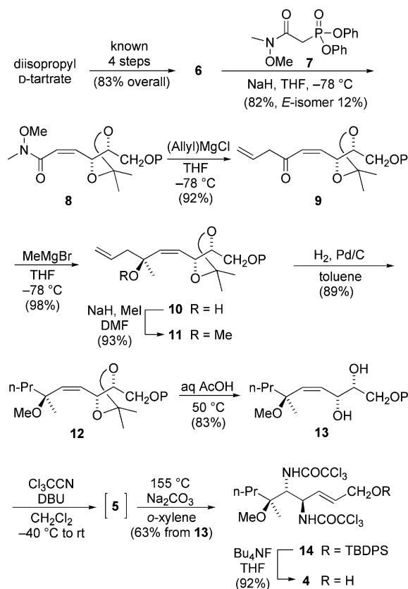
Scheme 1. P = TBDPS [ -\text{Si}(t\text{-Bu})\text{Ph}_2 ], allyl = \text{CH}_2=\text{CH}-\text{CH}_2- .
