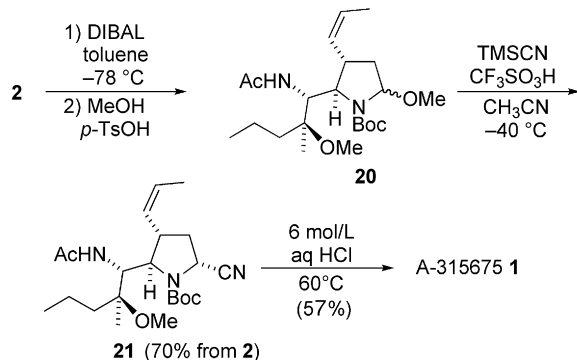
Scheme 3. DIBAL = diisobutylaluminum hydride, TMS = –SiMe 3 .
