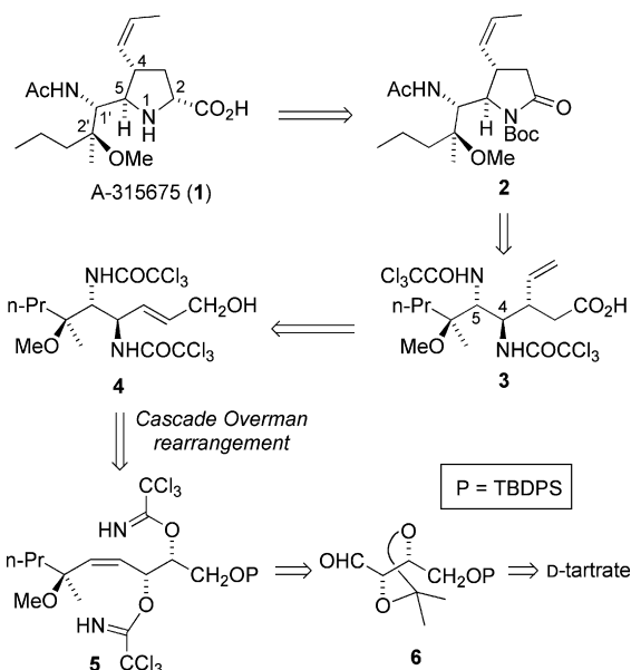
Fig. 1. Structure of A-315675 and its retrosynthetic analysis. TBDPS = -\text{SiPh}_2(t\text{-Bu}) , Boc = -\text{C}(\text{O})\text{O}(t\text{-Bu}) .
