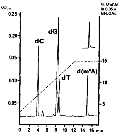
Fig. 4. HPLC analysis of the enzymatic digestion of the hexamer d(GGm 6 ATCC) on a Alltech Econosphere (5 μm) C18 column (0.47 × 15 cm). Eluent: 12-min linear gradient (3–15%) of MeCN in 50mM NH 4 OAc (pH 7.0), flow rate 1 ml·min -1 . Lower part: dC, dG, dT, and d(m 6 A) indicate the peaks corresponding to 2'-deoxycytidine, 2'-deoxyguanosine, thymidine, and 2'-deoxy- N 6 -methyladenosine, respectively. Upper part: Reversed-phase HPLC of 2'-deoxy- N 6 -methyladenosine.
