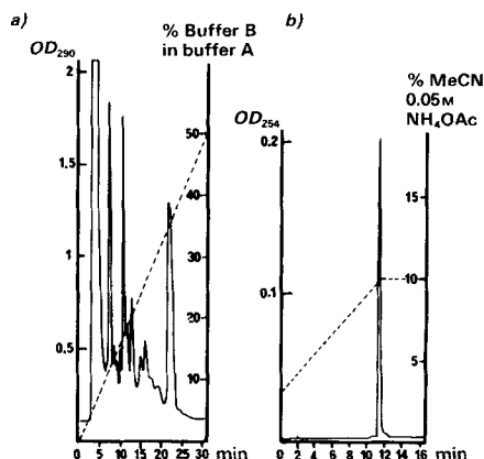
Fig. 3. HPLC profiles of oligonucleotide d(GGm 6 ATCC) . a) Crude mixture on Partisil 10 SAX (0.75 × 30 cm) with a 30-min linear gradient (0–50%) of buffer B (0.4M KH 2 PO 4 in H 2 O/MeCN 80:20 (v/v), pH 6.8) in buffer A (0.04M KH 2 PO 4 in the same solvent) at 2 ml·min -1 . b) Purified product on an Alltech Econosphere (5 μm) C18 column (0.47 × 15 cm) using a linear gradient (3–15%) of MeCN in 0.05M NH 4 OAc (pH 7.0) at 1 ml·min -1 .
