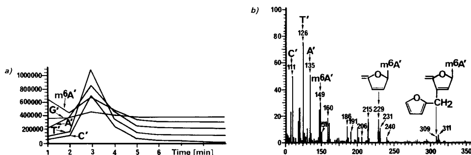
Fig. 5. Pyrolytic MS of the octanucleotide d (GGm 6 ATATCC). a ) Intensities of different ions against time during pyrolysis at 250°. b ) MS at 250° after 3 min of pyrolysis: A' = adenine, m 6 A' = N 6 -methyladenine, C' = cytosine, G' = guanine, and T' = thymine.
