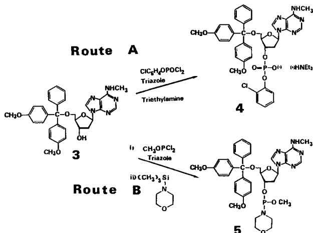
Scheme 2. Synthesis of the Protected Deoxyribonucleoside (Chlorophenyl phosphate) 4 (Route A) and of the Deoxyribonucleosid-3'-O-yl(methoxy)morpholinophosphate 5 (Route B)
