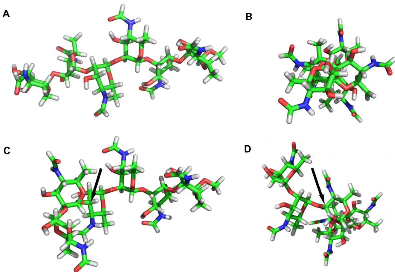
Figure 7. A) Side view of the A antigen; B) end on view of the rod-like conformation of the A antigen; C) side view of the M tetrasaccharide epitope attached to a 1,2-linked A type disaccharide; D) end on view of the hexasaccharide seen in (C). The A like character of the M antigen is seen in both side and end on views, except for the terminal disaccharide. All linkages are \alpha 1,2 except the \alpha 1,3 linkage indicated by the black arrows. The low energy conformations of the A and M antigens are based on glycosidic torsional angles previously reported. 11,31 The images displayed here were rendered with PyMOL Molecular Graphics System, Version 1.3 Schrödinger, LLC.
