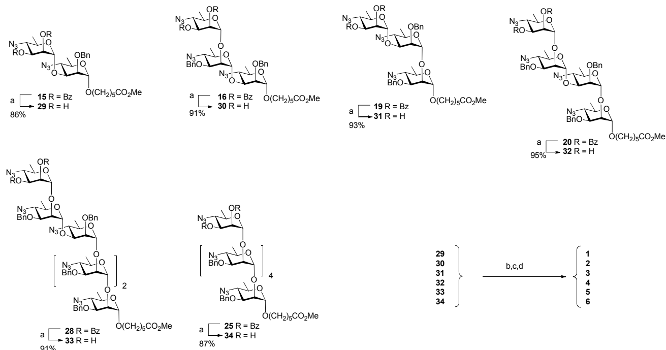
Scheme 5. Reagents and conditions: a) \text{NaOCH}_3 , \text{CH}_3\text{OH} , rt, 4 h; b) \text{H}_2\text{S} , \text{Py}/\text{H}_2\text{O} , 40 °C, 16 h; c) (\text{HCO})_2\text{O} , \text{CH}_3\text{OH} , -20 °C, 3 h; d) \text{H}_2 , \text{Pd}(\text{OH})_2 , \text{CH}_3\text{OH}/\text{H}_2\text{O} , rt, 16 h.
