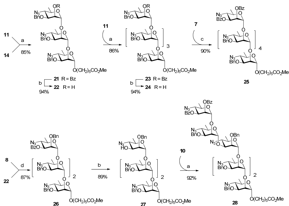
Scheme 4. Reagents and conditions: a) MeOTf, 3 Å MS, CH 2 Cl 2 , rt, 48 h; b) NaOCH 3 , CH 3 OH, rt, 4 h; c) TMSOTf, 3 Å MS, CH 2 Cl 2 , rt, 1 h; d) TMSOTf, 3 Å MS, PhMe, 95 °C, 1 h.
