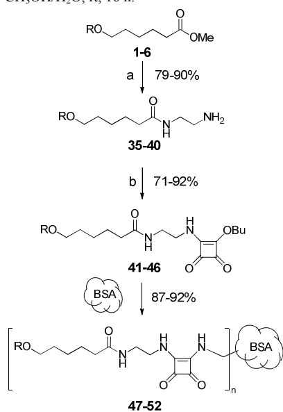
Scheme 6. Reagents and conditions: a) \text{NH}_2\text{CH}_2\text{CH}_2\text{NH}_2 , 20 °C, 48 h; b) dibutyl squarate, \text{EtOH}/\text{H}_2\text{O} , rt, 0.5 h; c) Borate buffer 0.5M, pH 9.0, rt, 72 h.
