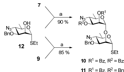
Scheme 1. Reagents and conditions: a) TMSOTf, 3Å MS, CH 2 Cl 2
