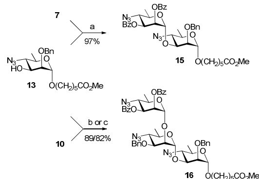
Scheme 2. Reagents and conditions: a) TMSOTf, 3Å MS, CH 2 Cl 2 , rt, 1 h; b) MeOTf, 3Å MS, CH 2 Cl 2 , rt, 48 h; c) NIS/AgOTf, 3Å MS, CH 2 Cl 2 , rt, 1 h.
