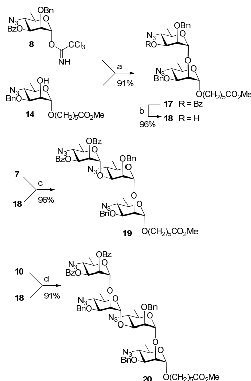
Scheme 3. Reagents and conditions: a) TMSOTf, 3 Å MS, PhMe, 95 °C, 1 h; b) NaOCH 3 , CH 3 OH, rt, 4 h; c) TMSOTf, 3 Å MS, CH 2 Cl 2 , rt, 1 h; d) MeOTf, 3 Å MS, CH 2 Cl 2 , rt, 48 h.
