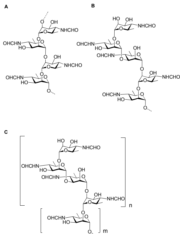
Figure 1. A) Structure of the B. abortus and Y. enterocolitica O:9 O-PS determined in 1984; 10,17 [ \rightarrow 2]Rha4NFo(1-) n ; B) Structure of the B. melitensis M antigen proposed in 1987; 11 C) Recently revised structure of the Brucella O-antigen with a capping M epitope terminating an A type \alpha 1,2-linked D-Rha4NFo polymer, where usually m \leq 16 . 15 The capping tetrasaccharide occurs a minimum of once, n = 1 or may be repeated several times, n > 1 .
