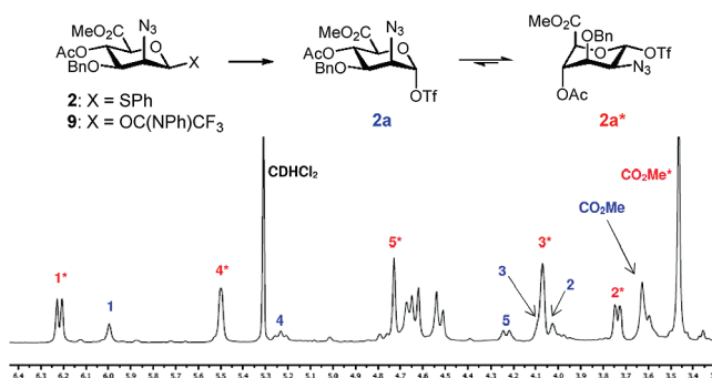
Figure 1. Part of the ^1\text{H} NMR spectrum obtained after activation of mannuronic acid esters 2 and 9 at -80^\circ\text{C} .
