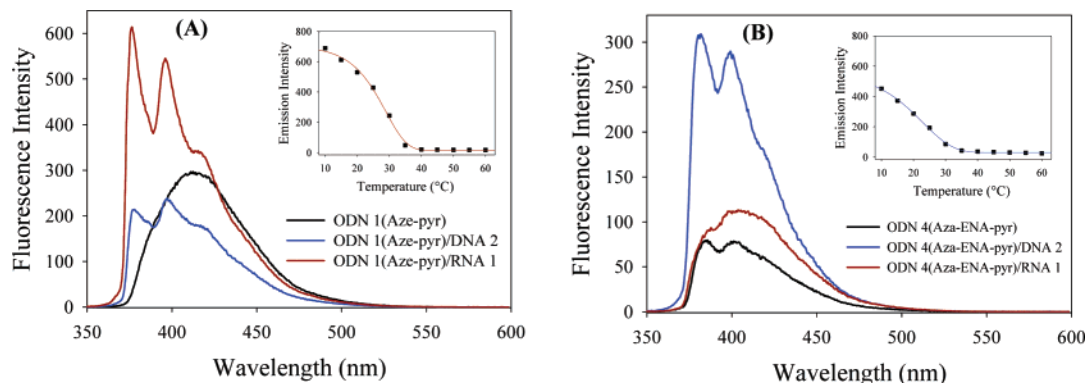
FIGURE 3. Fluorescence emission spectra of (A) Aze-pyr (X)-modified ODN 1 and (B) Aza-ENA-pyr (Y)-modified ODN 4 and the corresponding duplexes with complementary DNA 2 or RNA 1 targets. The temperature-dependent fluorescence changes (A) at 376 nm for the X-modified ODN 1/RNA 1 duplex and (B) at 385 nm for the Y-modified ODN 4/DNA 2 duplex are shown in the inset. Spectra were recorded at a total strand concentration of 0.8 \mu M and with an excitation wavelength of 340 nm.
