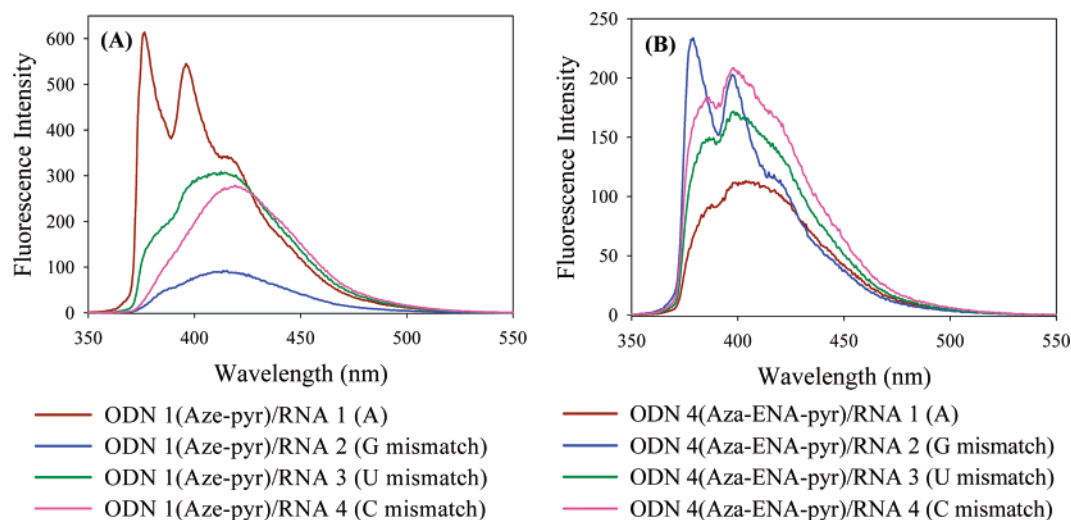
FIGURE 4. Fluorescence emission spectra of (A) Aze-pyr (X)-modified ODN 1 and (B) Aza-ENA-pyr (Y)-modified ODN 4 hybridized to the complementary RNA 1 and single base mismatch (G, U, or C) RNA 2, RNA 3, and RNA 4, respectively. Spectra were recorded at a total strand concentration of 0.8 \mu M and with an excitation wavelength of 340 nm.
