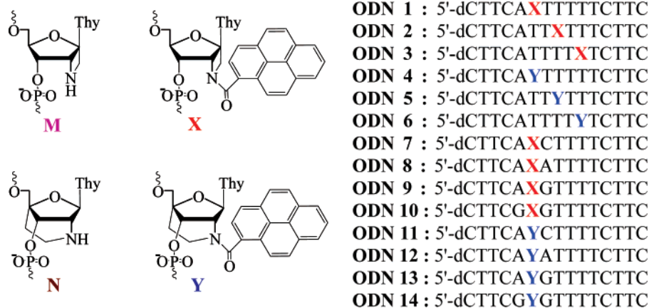
FIGURE 1. Structures of azetidine thymidine [Azetidine (M)], 2'-N-(pyren-1-yl)carbonyl-azetidine thymidine [Aze-pyr (X)], aza-ENA thymidine [Aza-ENA (N)], and 2'-N-(pyren-1-yl)carbonyl-aza-ENA thymidine [Aza-ENA-pyr (Y)] monomers are shown. Modified oligodeoxynucleotide sequences (ODNs 1–14) used in this study are also listed. For a complete list of oligonucleotides, see Table S1 in the Supporting Information.
