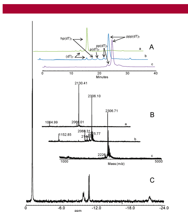
Figure 1. (A) Ion-exchange HPLC profiles of (a) crude hp(dT) 7 , (b) crude 5 , and (c) pure 5 . (B) Negative-mode MALDI-TOF MS profiles of (a) crude hp(dT) 7 , calcd m/z 2130.40, found 2130.41; (b) crude 5 , calcd m/z 2306.35, found 2306.10; (c) pure 5 , found 2306.70. (C) 31 P NMR spectrum of 5 . hp = 5'- H -phosphonate; p = 5'-phosphate; pp = 5'-diphosphate; ppp = 5'-triphosphate. Note: the large peak around 0 ppm is due to a signal from the phosphodiester linkages.
