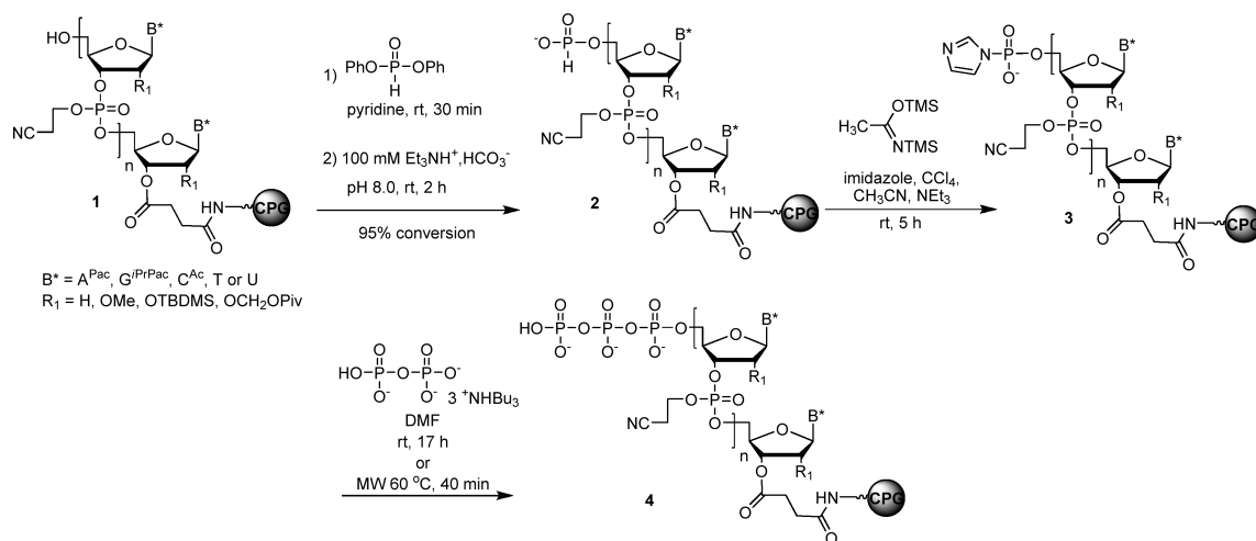
Scheme 1. General Synthesis of ON 5'-TPs on Solid Support
