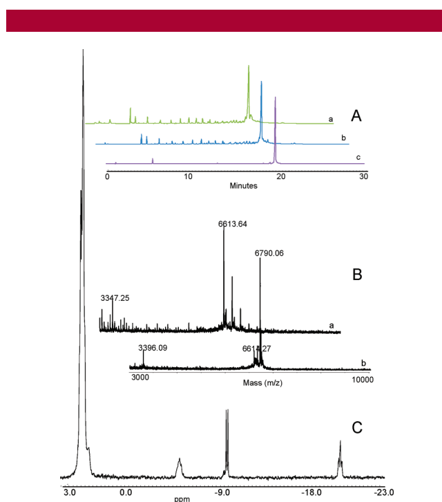
Figure 2. (A) Ion-exchange HPLC profiles of (a) crude hpUUGUCUCUGGUCCUUAACUUA; (b) crude 8 ; (c) pure 8 . (B) MALDI-TOF MS profiles of (a) crude hpUUGUCUCUGGUCCUUAACUUA, calcd m/z 6611.87, found 6613.64; (b) pure 8 , calcd m/z 6787.87, found 6790.06. (C) 31 P NMR spectrum of 9 .
