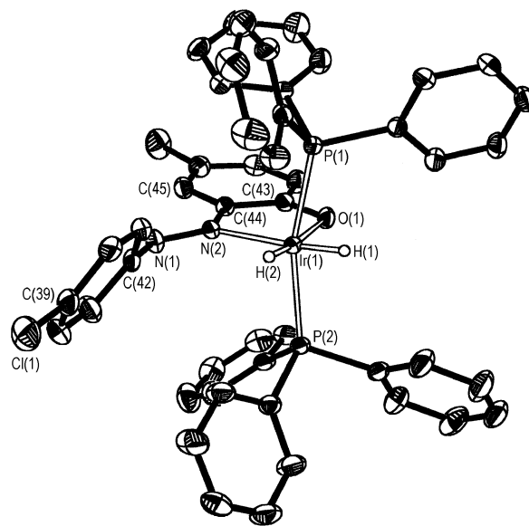
Figure 2. View of the [\text{Ir}(\text{PPh}_3)_2(\text{NO}-\text{Cl})(\text{H})_2] complex.
