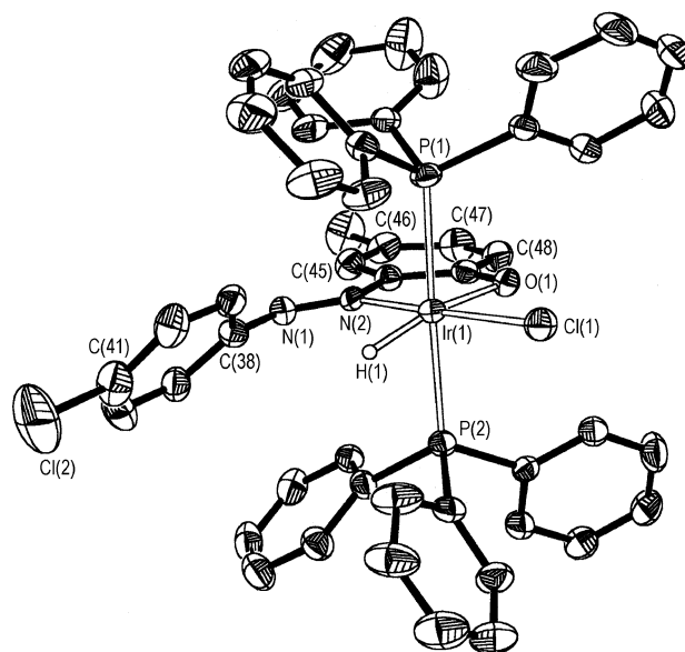
Figure 1. View of the [\text{Ir}(\text{PPh}_3)_2(\text{NO}-\text{Cl})(\text{H})\text{Cl}] complex.
