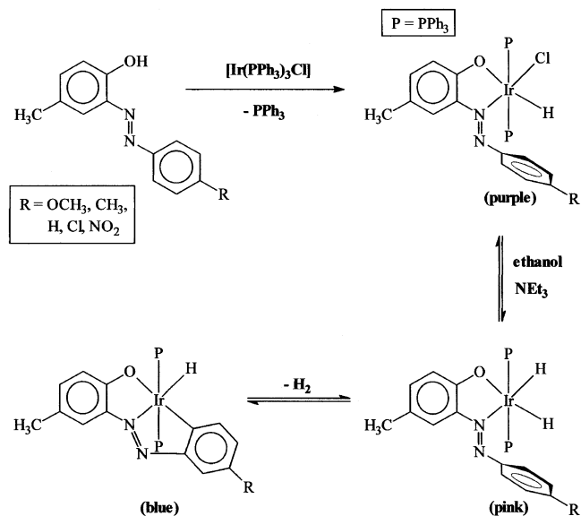
Scheme 1. Probable Steps of the Reaction in Ethanol
