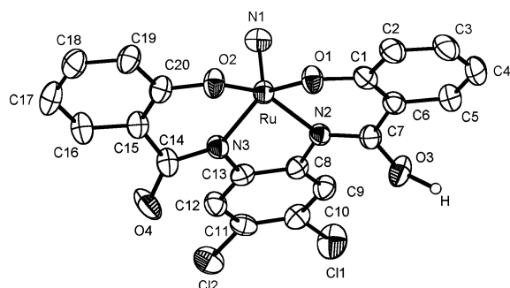
Fig. 9 Perspective view of [\text{Ru}^{\text{VI}}(\text{N})(\text{HL}^2)] ( 7 ) with atom labelling scheme (50% probability ellipsoids).
