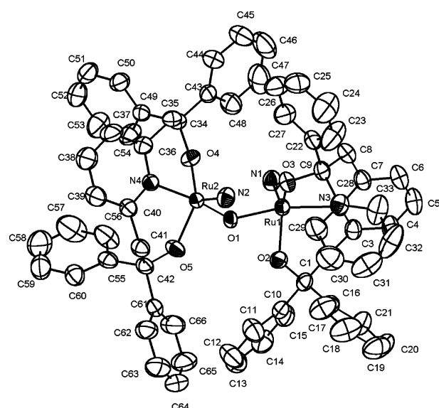
Fig. 8 Perspective view of the complex cation of [\text{Ru}_2(\text{N})(\text{L}^1)_2(\mu\text{-OH})]\text{PF}_6 ( 6 ) with atom labelling scheme (50% probability ellipsoids).
