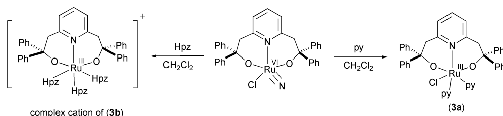
Scheme 2 Reactions in the \text{py-CH}_2\text{Cl}_2 and \text{Hpz-CH}_2\text{Cl}_2 solutions.
