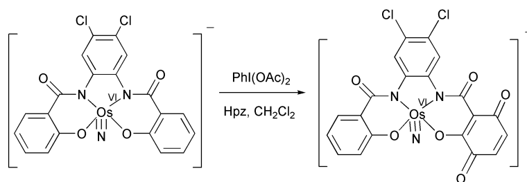
complex anion of 8
