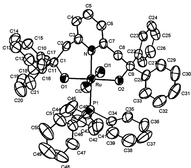
Fig. 2 Perspective view of [\text{Ru}^{\text{III}}(\text{HL}^1)(\text{PPh}_3)_2\text{Cl}] ( 2a ) with atom labelling scheme (50% probability ellipsoids).
