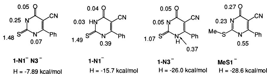
Figure 1. Calculated (PM3-AQ) HOMO electron densities for anions derived from 1 (Ar=Ph) and MeS1 by deprotonation at the indicated sites. H denotes the calculated heat of formation
