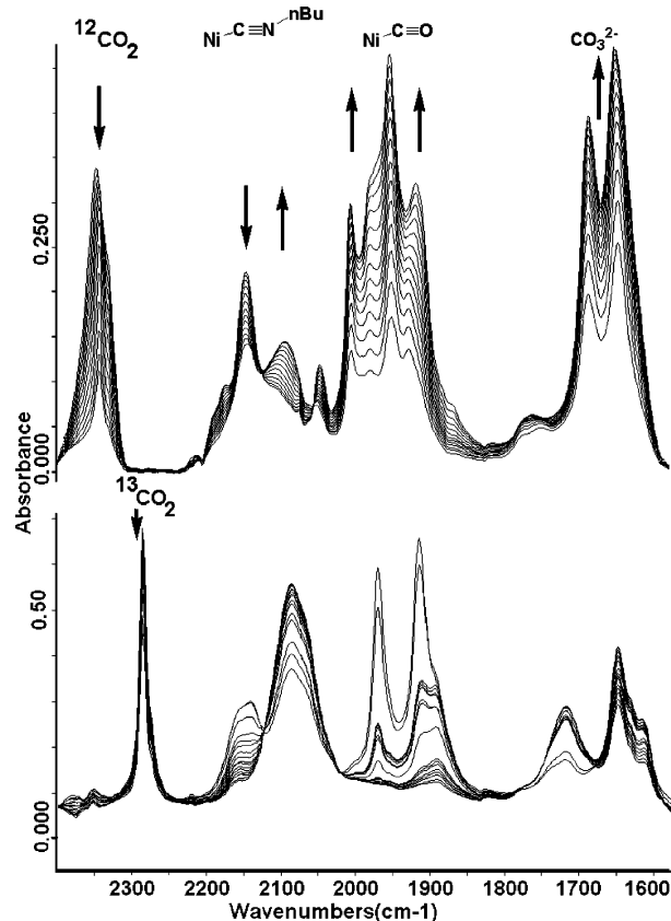
Figure 5. Observed changes in the IR (2500–1600 \text{cm}^{-1} ) spectrum during the bulk electrolysis at -1.3 V of [\text{Ni}_2(\mu_2\text{-dppa})_2(\mu_2\text{-n-BuNC})(\text{n-BuNC})_2] ( 2 ) in the presence of \text{CO}_2 (SEC) ( ^{12}\text{CO}_2 , top; ^{13}\text{CO}_2 , bottom).
