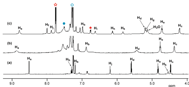
Figure 2. ^1\text{H} NMR spectra (600 MHz, \text{CDCl}_3 ) of (a) 1 alone at 298 K; (b) [\mathbf{1}] = [\mathbf{2}] = 4.5 \text{ mM} at 298 K (capsule 3 ); and (c) [\mathbf{1}] = [\mathbf{2}] = 4.5 \text{ mM} and [\text{TBAOTf}] = [\mathbf{4}] = 11.2 \text{ mM} at 253 K.
