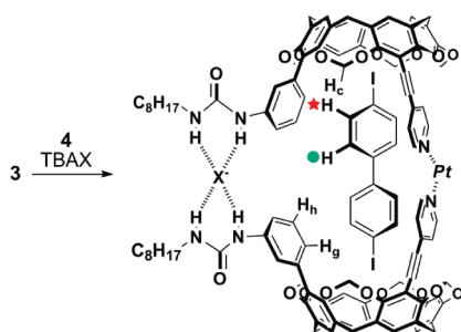
Figure 3. Structure of 4 -encapsulated hybrid capsule 3 with anion assistance.
