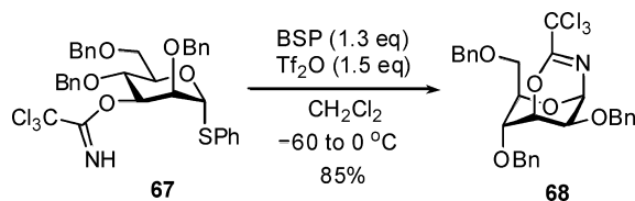
Scheme 1. Formation of 68 by Intramolecular Trapping of the Anomeric Oxocarbenium Ion Intermediate Resulting from the Activation of 67
