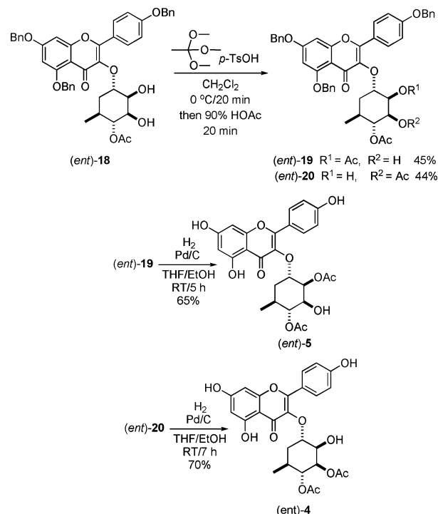
Scheme 9. Synthesis of ent - 5 and ent - 4
