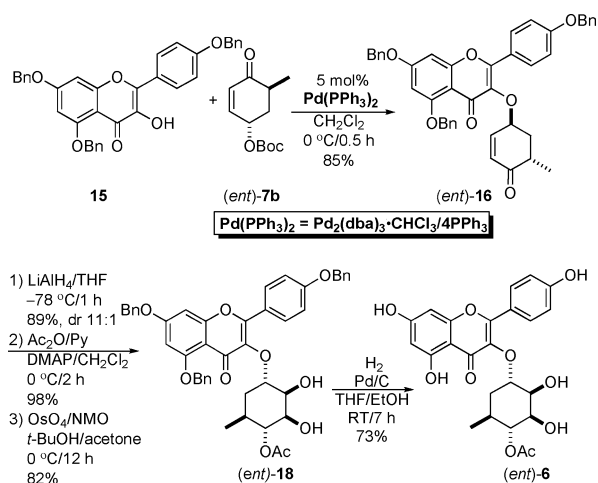
Scheme 8. Synthesis of ent - 6
