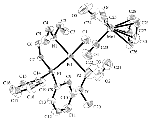
Figure 4. ORTEP drawing of [PtMe{P(OMe) 3 }(Et 2 NC 2 H 4 PPh 2 - \kappa^2 N,P)] + [MoCp(CO) 3 ] - ( 21 ). All hydrogen atoms are omitted for clarity. Ellipsoids represent 50% probability.
