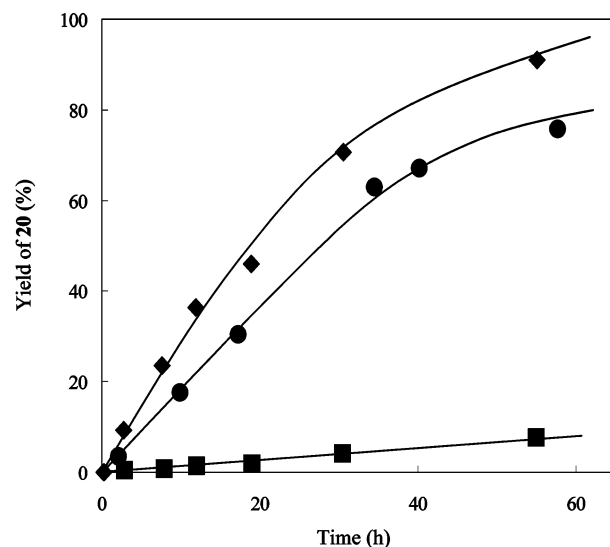
Figure 5. Time-yield curves for trans-cis isomerization from 22 to 20 . Conditions: temp = 30 °C, [ 22 ] = 1.5 \times 10^{-2} M, solvent = \text{CD}_3\text{COCD}_3 . [ \text{PPh}_3 ]/[ 22 ] = 0 (■), 2 (●), 4 (◆).
