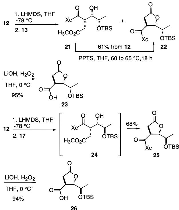
Scheme 3
