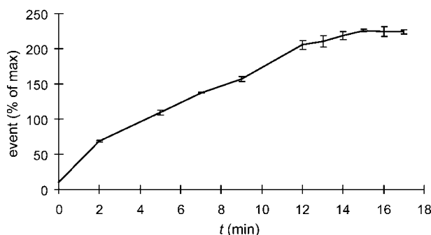
Figure 3. Analysis of CuAAC kinetics on the surface of CHO cells by flow cytometry. CHO cells were incubated for 3 days in untreated medium or medium supplemented with 50 μM Ac 4 ManNAz, followed by labeling with 100 μM biotin-alkyne in the presence of BTES-Cu(I) catalyst ([Cu] = 75 μM). The reaction was quenched at various time points with BCS and probed with Alexa Fluor 488-streptavidin conjugates. Error bars represent the standard deviation of three replicate experiments.
