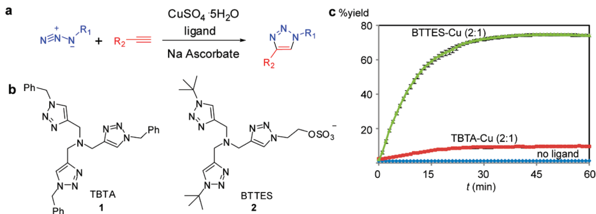
Figure 1. Copper(I)-catalyzed azide–alkyne cycloaddition (CuAAC) is accelerated by Cu(I)-stabilizing ligands. (a) CuAAC of azides and terminal alkynes to form 1,4-disubstituted 1,2,3-triazoles. (b) Structures of CuAAC-accelerating ligands. (c) Conversion–time profiles of CuAAC in the presence/absence of accelerating ligands. Reaction conditions: propargyl alcohol (50 \mu M), 3-azido-7-hydroxy-coumarin (100 \mu M), \text{CuSO}_4 (75 \mu M), 0.1 M potassium phosphate buffer (pH 7.0)/DMSO 95:5, sodium ascorbate (2.5 \mu M), room temperature. Error bars represent the standard deviation of three replicate experiments.
