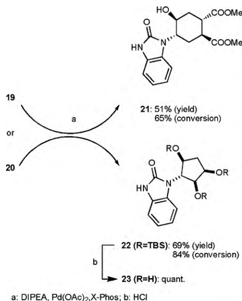
Scheme 6. Synthesis of benzimidazolones 21 and 23 .
