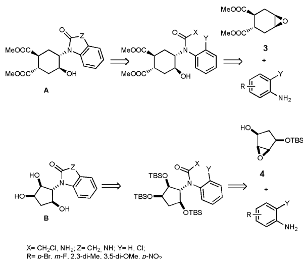
Chart 1. General structures of the targets and retrosynthetic approaches.
