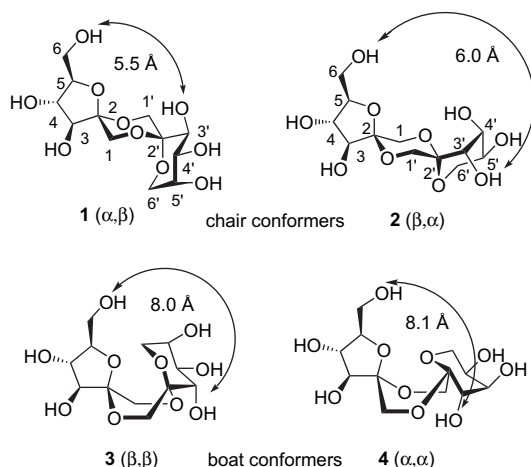
Figure 2. Conformations of the different type II DFA diastereomers with indication of the O-6–O-3' interatomic distance.
