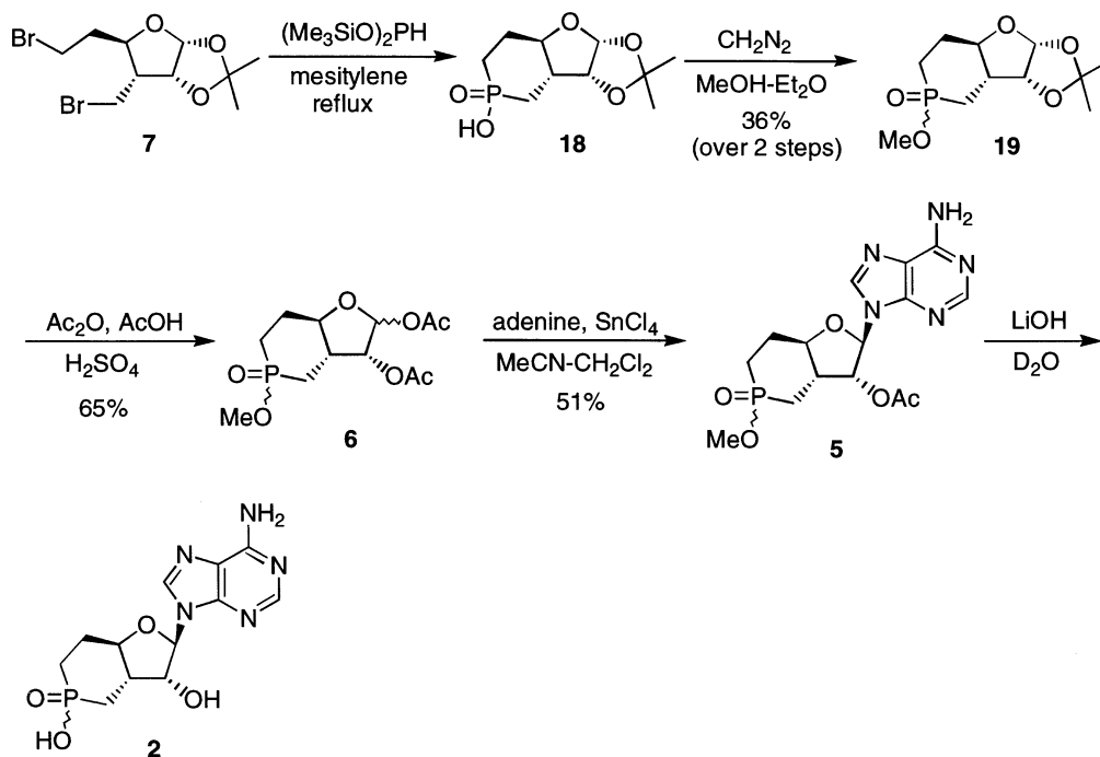
Scheme 3.
