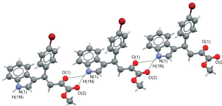
Figure 2. The infinite molecular chain adopted in the solid state by ( R )- 4m as determined by X-ray structure studies. Features of the N–H⋯O interactions are: \text{N}(1)\cdots\text{O}(1) 3.31(1) Å, \text{H}(1\text{N})\cdots\text{O}(1) 2.53(3) Å, \text{N}(1)\cdots\text{O}(2) 3.03(1) Å, \text{H}(1\text{N})\cdots\text{O}(2) 2.17(4) Å, \text{N}(1)\cdots\text{H}(1\text{N})\cdots\text{O}(2) 150(2) ^{\circ} .
