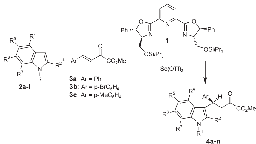
Scheme 2. The scandium triflate complex of 1 as a chiral catalyst in the Friedel–Crafts reactions between 2a–I and 3a–c , which give 4a–n after chromatographic purification.
