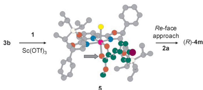
Figure 3. The assumed reactive intermediate 5 of the Friedel–Crafts alkylation reaction between 3b and indole 2a catalyzed by the \text{Sc}(\text{OTf})_3 complex of pybox 1 , which gives ( R )- 4m .
