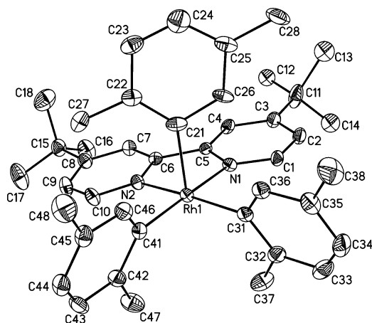
Figure 2. Molecular structure of \text{Rh}(\text{dtbpy})(\text{C}_8\text{H}_9)_3 ( 6 ). The ellipsoids are drawn at 40% probability level.
