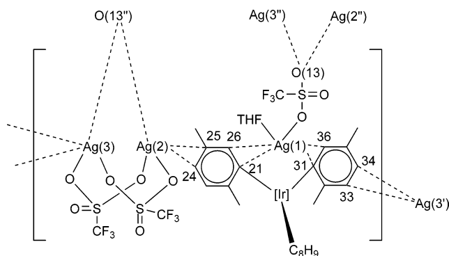
Figure 4. Molecular structure of \text{Ir}(\text{dtbpy})(\text{C}_8\text{H}_9)_3(\text{CNxyI}) ( 8 ). The ellipsoids are drawn at 40% probability level.
