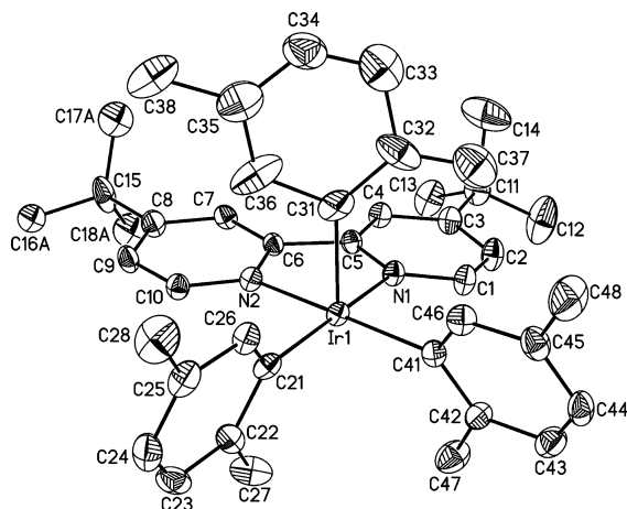
Figure 3. Molecular structure of \text{Ir}(\text{dtbpy})(\text{C}_8\text{H}_9)_3 ( 7 ). The ellipsoids are drawn at 40% probability level.
