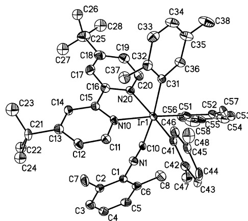
Figure 4. Molecular structure of \text{Ir}(\text{dtbpy})(\text{C}_8\text{H}_9)_3(\text{CNxyI}) ( 8 ). The ellipsoids are drawn at 40% probability level.
