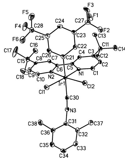
Figure 7. Molecular structure of \text{Ir}(\text{dtbpy})(\text{Ar}_\text{F})(\text{CNxyl})\text{Cl}_{1.4}\text{Br}_{0.6} ( 11 ). A disorder of the two halide sites was found. Only positions of the chlorides Cl(1) and Cl(2) are shown. The ellipsoids are drawn at 40% probability level.
