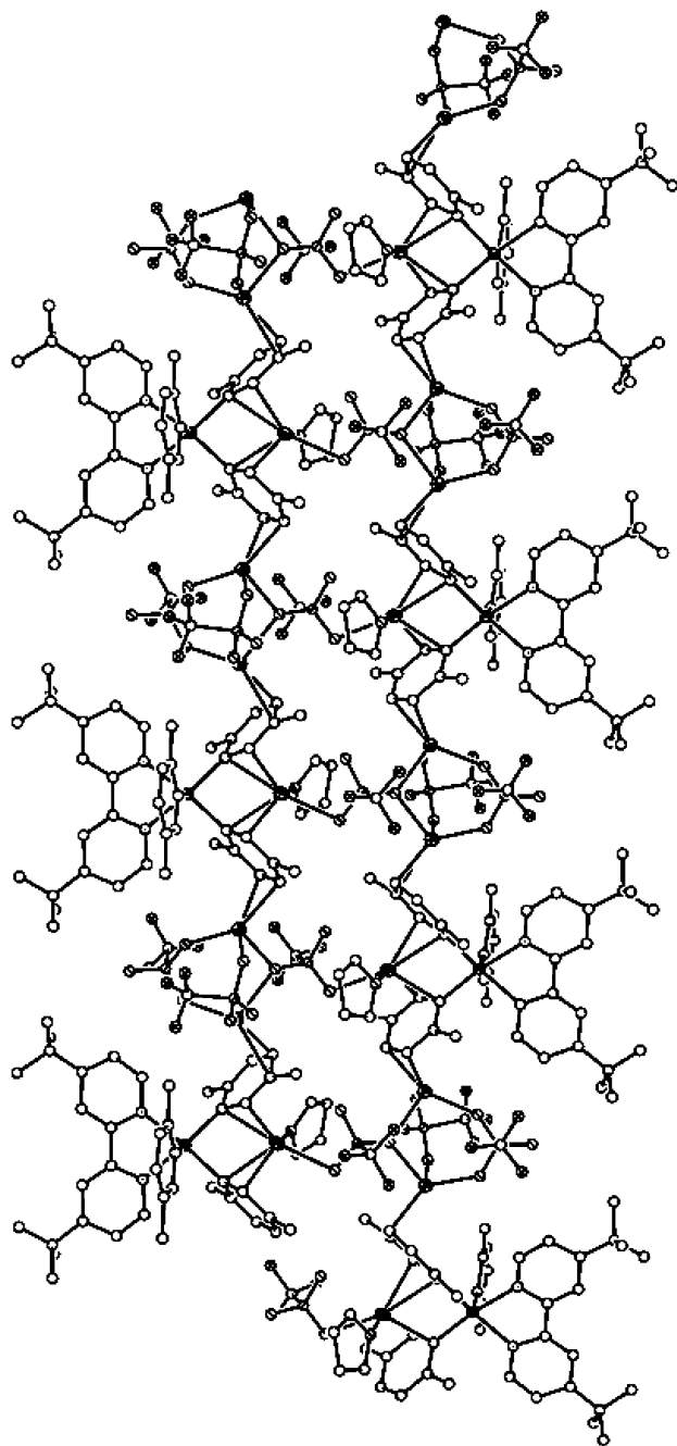
Figure 5. Double-chain structure of [\text{Ir}(\text{dtbpy})(\text{C}_8\text{H}_9)_3\{\text{Ag}(\text{OTf})(\text{THF})\}\{\text{Ag}_2(\text{OTf})_2\}]_\infty ( 9 ).
