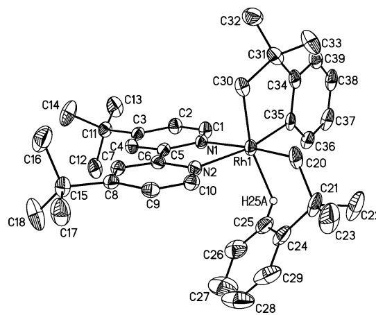
Figure 1. Molecular structure of \text{Rh}(\text{dtbpy})(\text{CH}_2\text{CMe}_2\text{C}_6\text{H}_4)(\text{CH}_2-\text{CMe}_2\text{Ph}) ( 2 ). The ellipsoids are drawn at 40% probability level.
