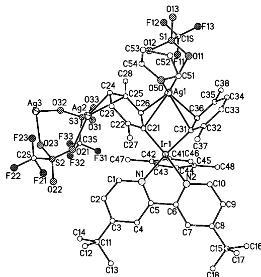
Figure 6. Structure of the repeat unit \text{Ir}(\text{dtbpy})(\text{C}_8\text{H}_9)_3\{\text{Ag}(\text{OTf})(\text{THF})\}\{\text{Ag}_2(\text{OTf})_2\} in 9 showing atom-labeling schemes of selected atoms. The prime and double-prime notations are used to indicate atoms in an adjacent repeat unit of the same chain and those in the adjacent chain, respectively.
