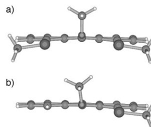
Figure 7. Optimized structures of a) 4 (BB) and b) 10 (B) . The optimized torsional angles ( \varphi(C_1C_9OC_{Me}) ) for 4 (BB) and 10 (B) are 94.3^\circ and 101.7^\circ , respectively.
